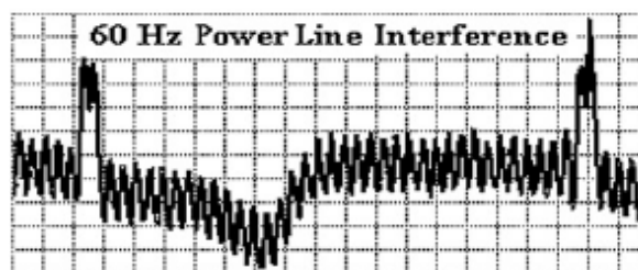
Fig. 4 60Hz power-line interference
