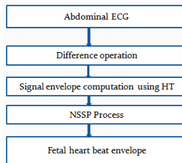
Fig. 1 Block diagram.
